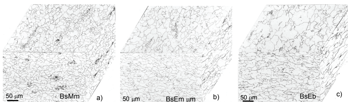
Fig 4. Microstructure of the coil with thickness 0.8 a) middle of the coil, middle of the strip b)middle of the coil; edge of the strip c) beginning of the coil, edge of the strip
