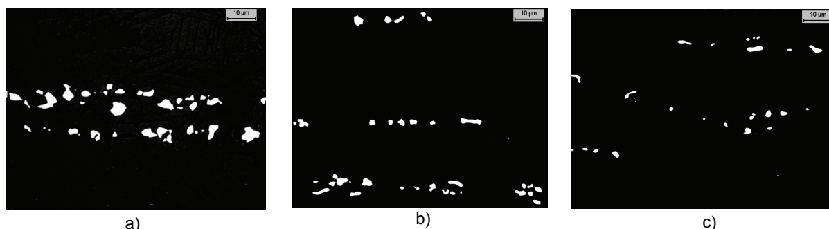
Fig. 7 Carbides morphology on longitudinal section; Klemm'I a) AaMm; b) AaEm; c) AaEe;
