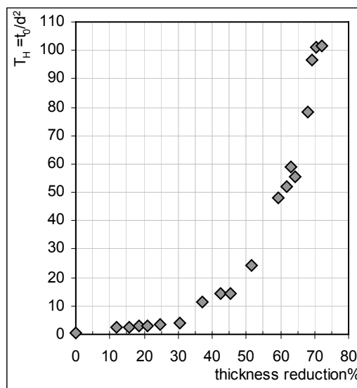
Fig.1 The cold rolling effect on the hydrogen permeation time
